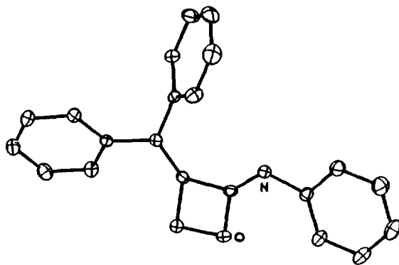
Figure. A perspective view of compound 2a .
